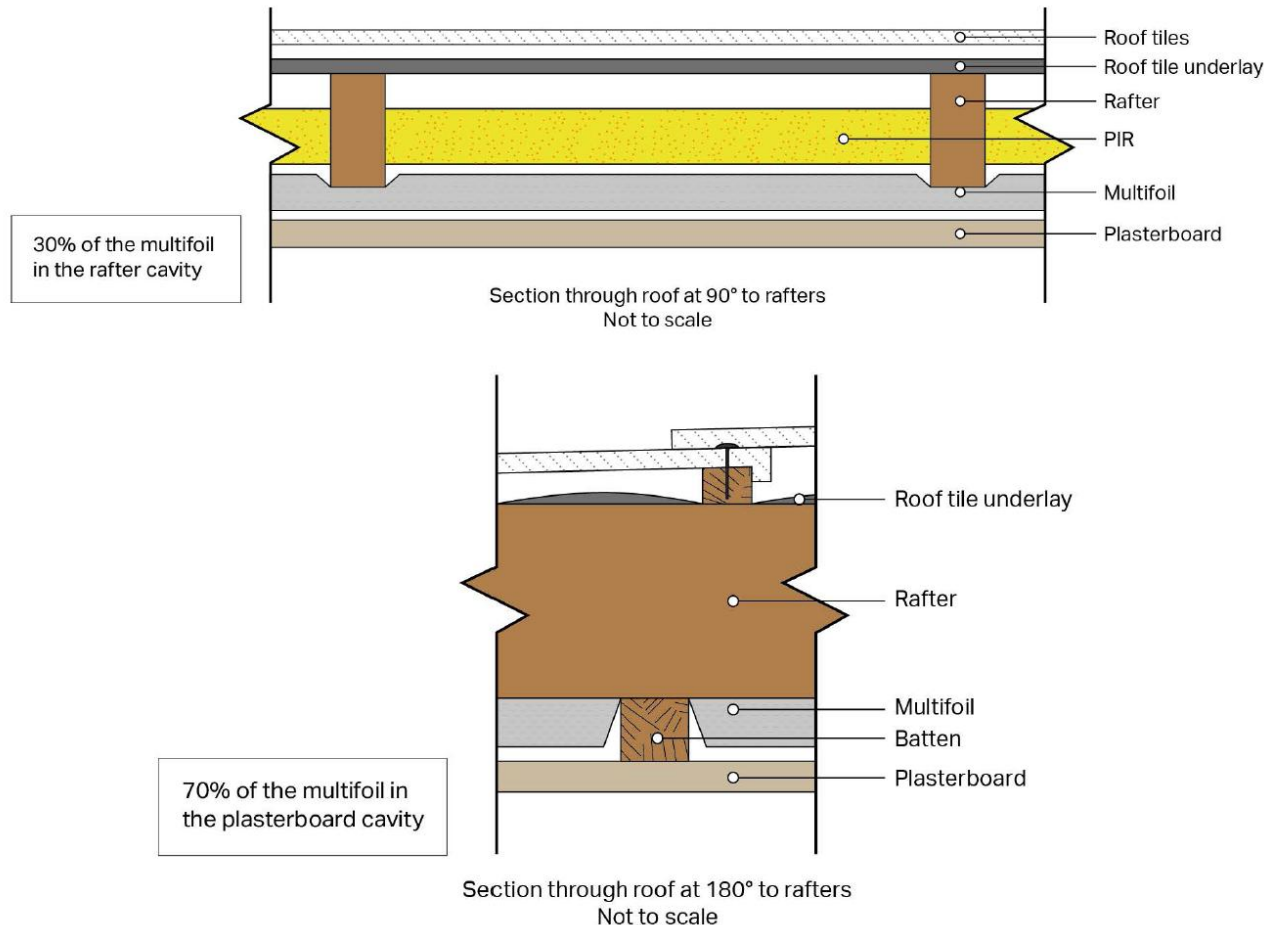
Figure 1 Roof construction using reflective insulation and PIR
