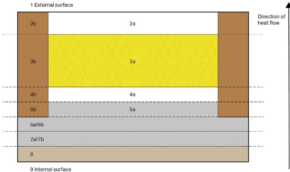
Figure 2 Schematic of roof construction (not to scale)
